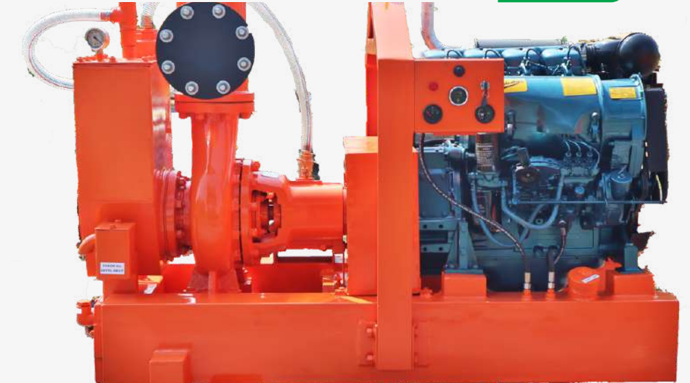
8 inch dewatering pump
